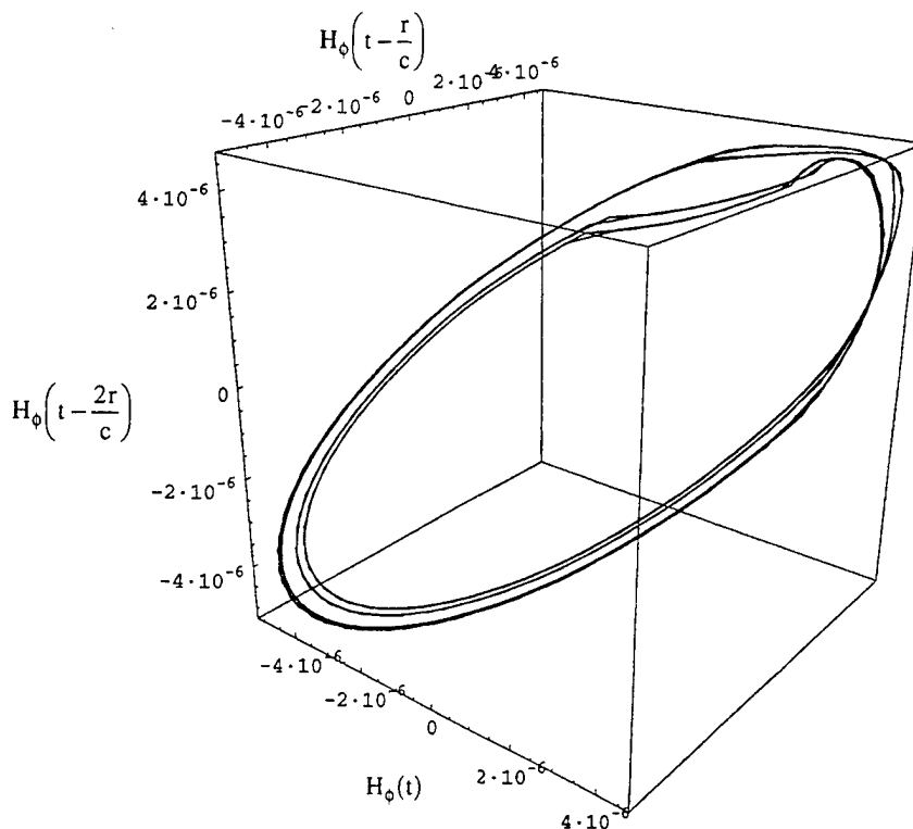
(a) Three-dimensional delay coordinate plot of magnetic field, H_\phi . Circuit parameters are R_0 = 12.5 \Omega , L = 18.0 \text{ mH} , C_1 = 10.0 \text{ nF} , C_2 = 100.0 \text{ nF} , G_a = -757.576 \mu\text{S} , G_b = -409.090 \mu\text{S} , E = 1.0 \text{ V} , C_a = 10.0 \text{ pF} , G = 539.0 \mu\text{S} , r = 7.5 \times 10^3 \text{ m} , h = 0.01 \text{ m} , \theta = \pi/2 , I_a = 100 \text{ A} , c = 3 \times 10^8 \text{ m/s} .
