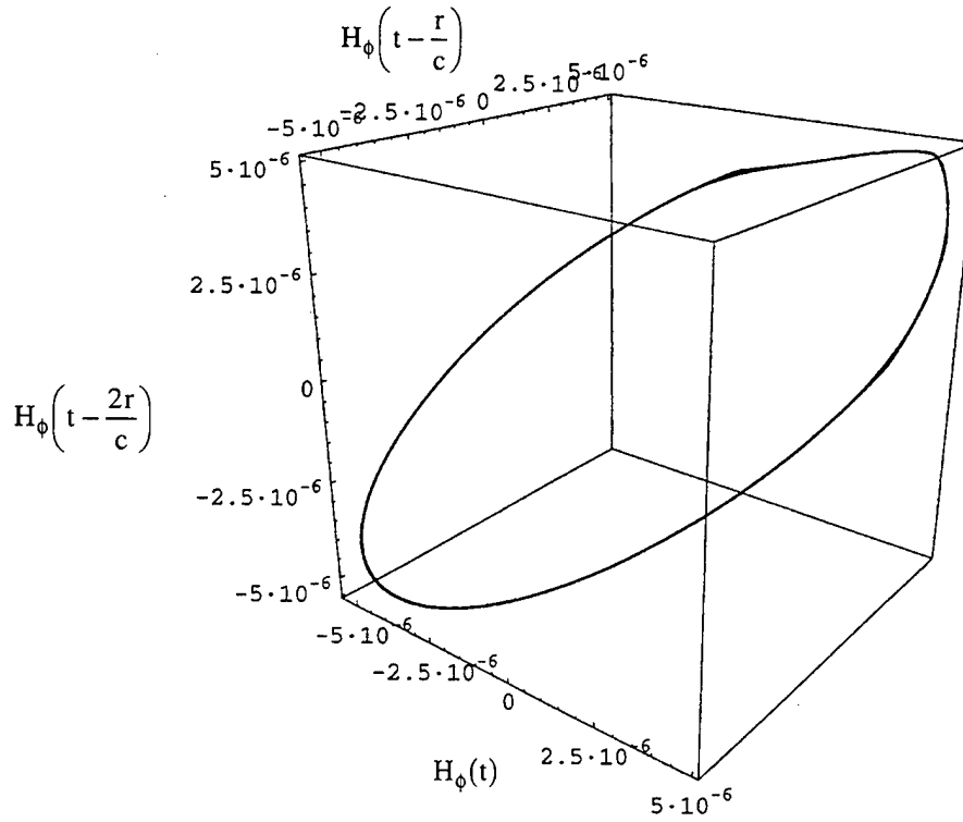
(a) Three-dimensional delay coordinate plot, H_\phi . Circuit parameters are R_0 = 12.5 \Omega , L = 18.0 \text{ mH} , C_1 = 10.0 \text{ nF} , C_2 = 100.0 \text{ nF} , G_a = -757.576 \mu\text{S} , G_b = -409.090 \mu\text{S} , E = 1.0 \text{ V} , C_a = 10.0 \text{ pF} , G = 530.0 \mu\text{S} , r = 7.5 \times 10^3 \text{ m} , h = 0.01 \text{ m} , \theta = \pi/2 , I_0 = 100 \text{ A} , c = 3 \times 10^8 \text{ m/s} .
