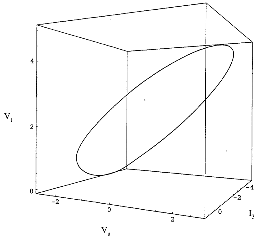
(a) Three-dimensional phase space plot of antenna voltage versus V_1 and I_3 . Circuit parameters are R_0 = 12.5 \Omega , L = 18.0 \text{ mH} , C_1 = 10.0 \text{ nF} , C_2 = 100.0 \text{ nF} , G_a = -757.576 \mu\text{S} , G_b = -409.090 \mu\text{S} , E = 1.0 \text{ V} , C_a = 10.0 \text{ pF} , G = 530.0 \mu\text{S} .
