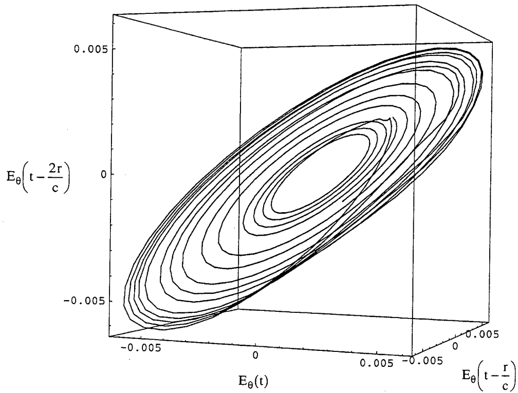
(a) Three-dimensional delay coordinate plot of electric field, E_\theta (same parameters as Figure 11a).
