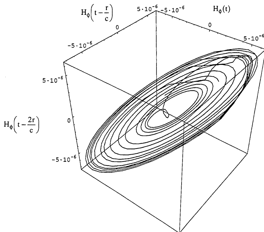
(a) Three-dimensional delay coordinate plot of magnetic field, H_\phi . Circuit parameters are R_0 = 12.5 \Omega , L = 18.0 \text{ mH} , C_1 = 10.0 \text{ nF} , C_2 = 100.0 \text{ nF} , G_a = -757.576 \mu\text{S} , G_b = -409.090 \mu\text{S} , E = 1.0 \text{ V} , C_a = 10.0 \text{ pF} , G = 550.0 \mu\text{S} , r = 7.5 \times 10^3 \text{ m} , h = .01 \text{ m} , \theta = \pi/2 , I_a = 100 \text{ A} , c = 3 \times 10^8 \text{ m/s} .
