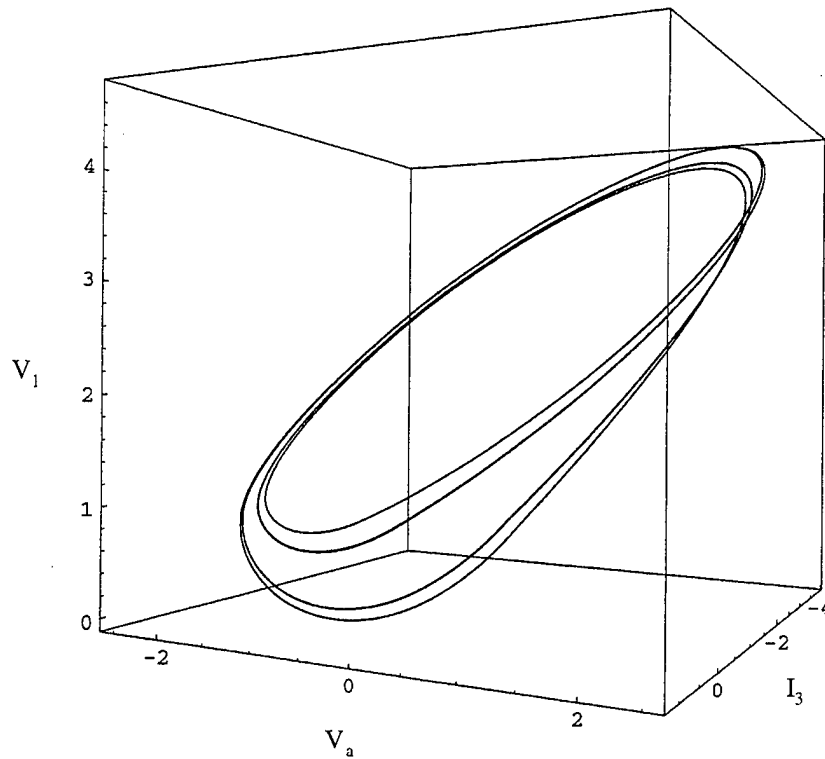
(a) Three-dimensional phase space plot of antenna voltage versus V_1 and I_3 . Circuit parameters are R_0 = 12.5 \Omega , L = 18.0 \text{ mH} , C_1 = 10.0 \text{ nF} , C_2 = 100.0 \text{ nF} , G_a = -757.576 \mu\text{S} , G_b = -409.090 \mu\text{S} , E = 1.0 \text{ V} , C_a = 10.0 \text{ pF} , G = 539.0 \mu\text{S} .
