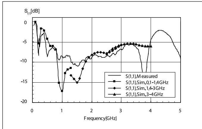
▲ Figure 4. Measured and simulated S_{11} -parameter for the CPW-fed spiral antenna on FR-4 substrate material.
