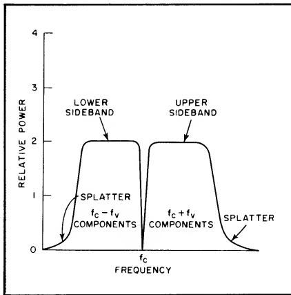
Figure 2: double sideband.
