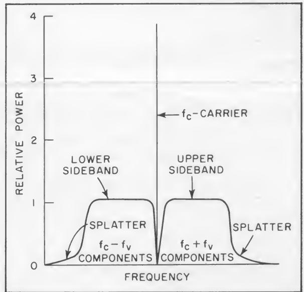
Figure 1: amplitude modulation.
