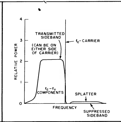
Figure 3: compatible SSB.
