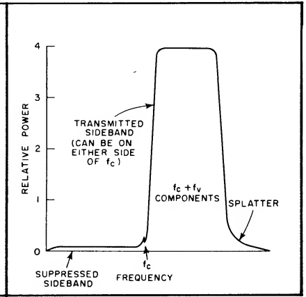
Figure 4: single sideband.
