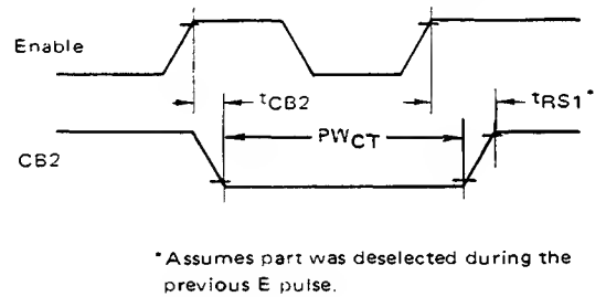
FIGURE 11 — CB2 DELAY TIME (Write Mode; CRB-5=CRB-3=1, CRB-4=0)
