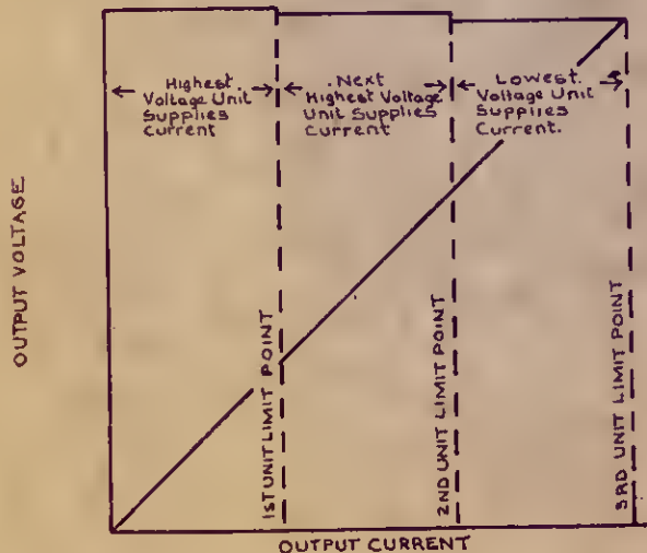
Fig 6. Parallel Operation
