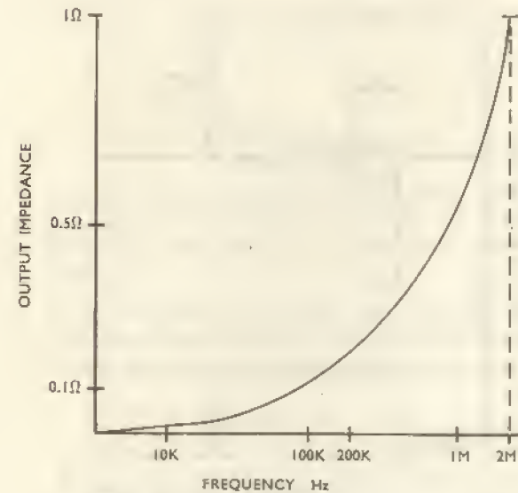
Fig. 2. Output Impedance
