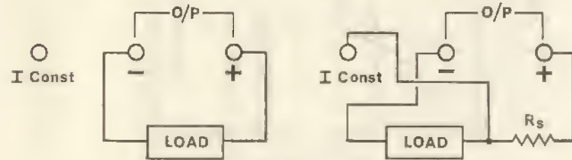
Fig. 1. CV and CI Connections
