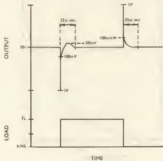
Fig. 4. Pulse Response
